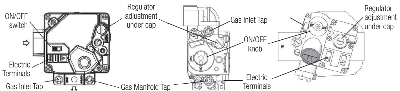
Figure 21: Gas Valves
