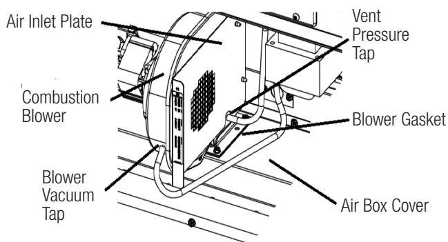
Figure 25: Combustion Blower
